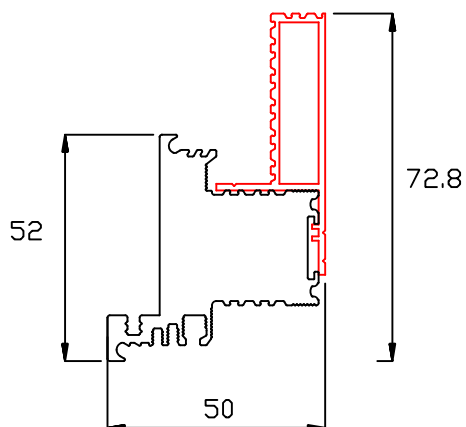
DETAIL M5:1
